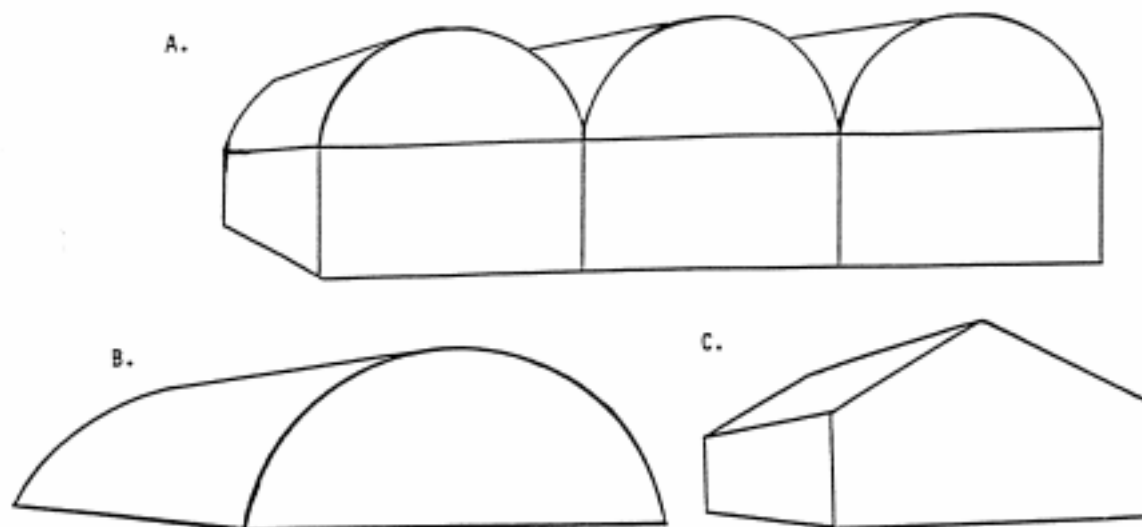
Figure 1. Commercial greenhouse structures: A) gutter connected, B) quonset, and C) single gable.
